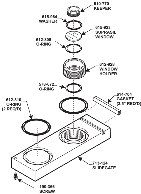
713-121 SLIDE WINDOW ASSEMBLY NOTE: For spectrometers with wavelengths <165 nm 612-807 (Suprasil) Window required.
